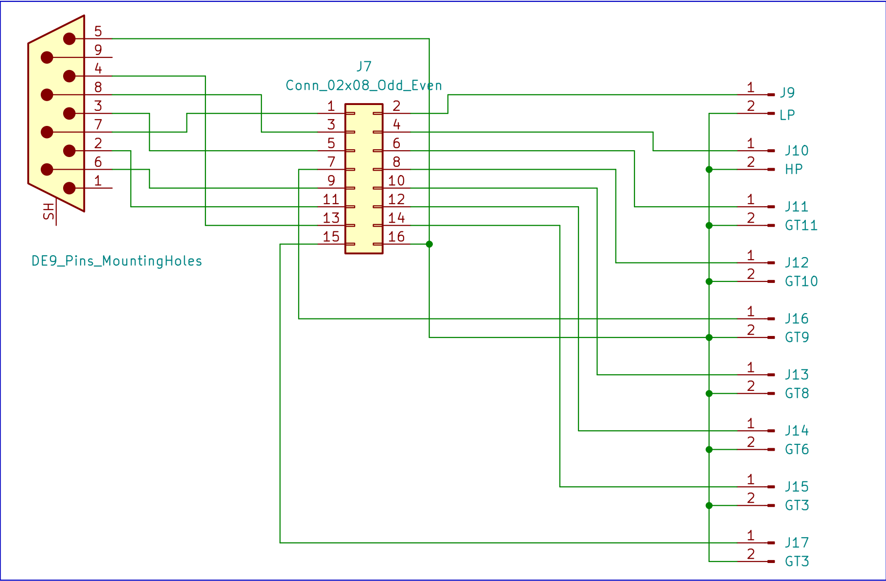
Internal Sensors/Service Port – PCB
