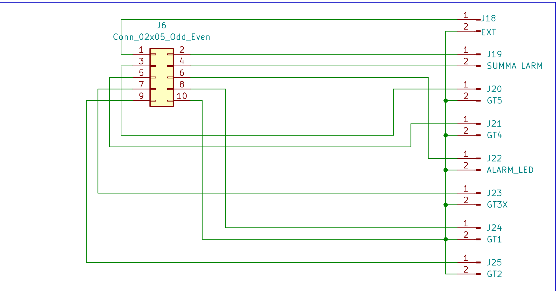
External Sensors/Ext Ctrl Inp/Larm Output – PCB
